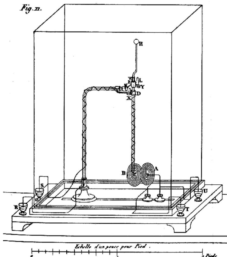
Figure 3.8: Ampère's first observation of attraction and repulsion between two current-carrying conductors. Spiral A remains fixed in the laboratory, while spiral B is mobile in such a way that it can move towards spiral A or away from it.
