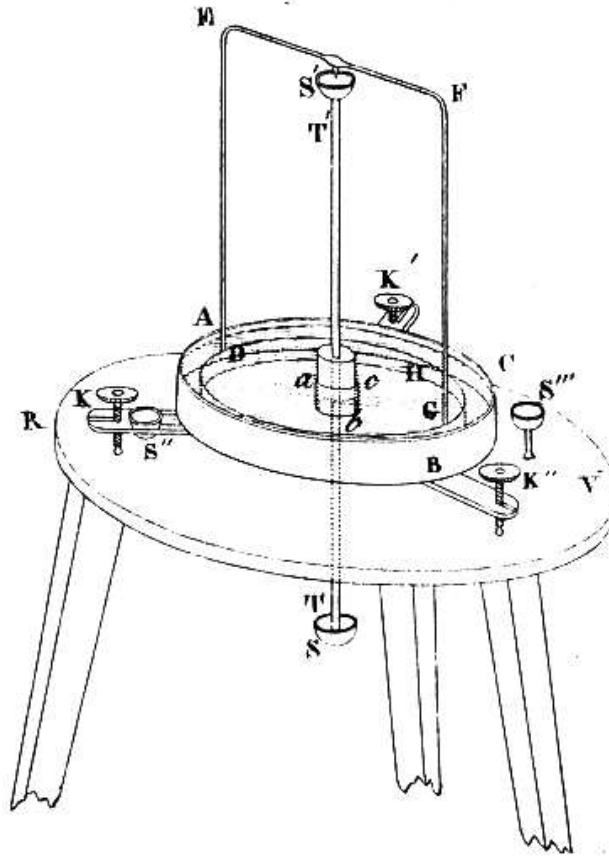
Figure 7.10: Ampère's instrument to obtain a continuous rotation utilizing only current-carrying conductors. He did not employ magnets or terrestrial magnetism.
