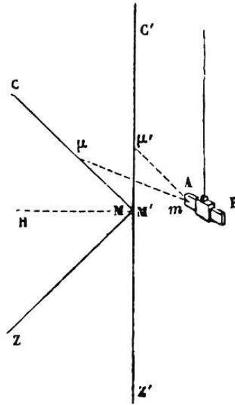
Figure 6.6: Biot and Savart's experiment with the bent wire. The current flows from the zinc Z towards the copper C , that is, in the direction Z'M'C' along the vertical wire, and in the direction ZMC along the bent wire located in this vertical plane. Points M and M' are electrically insulated from one another. The small magnetized needle AB can oscillate in a horizontal plane passing through HMM' around the vertical thread holding it. The letter m represents a magnetic pole of the needle, while \mu and \mu' represent small elements of the current-carrying wires.
