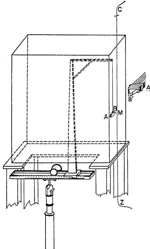
Figure 6.2: Biot and Savart's experiment with the straight wire. The electric current flows from Z to C . The small magnetized needle AB can oscillate in a horizontal plane around the vertical silk thread.
