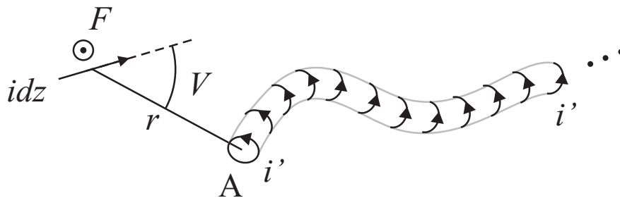
Figure 9.8: Interaction between a current element and an indefinite solenoid.
