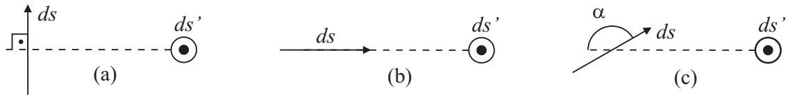
Figure 4.15: Ampère considered that the electrodynamic force between the current elements of lengths ds and ds' vanishes in these three configurations. The element ds' is orthogonal to the plane of the paper, with its center in this plane. The element ds , on the other hand, is located in the plane of the paper.
