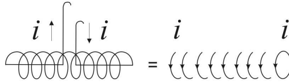
Figure 4.10: An axially compensated helix is equivalent to a purely circular or azimuthal current flowing over the surface of a cylinder, without a longitudinal or axial component.
