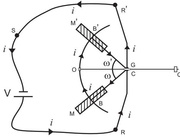
Figure 10.15: Arc BB' with its center C along the vertical rotation axis GH remains in equilibrium.
