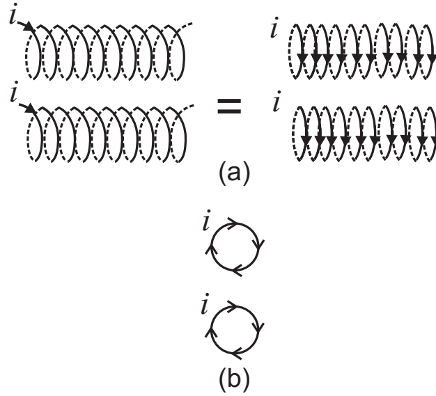
Figure 4.8: (a) Ampère expected initially that each one of these helices were equivalent to a cylinder in which the currents were flowing only along the azimuthal direction \varphi . (b) Cross sections of two side by side cylinders carrying azimuthal currents. The currents which are closer to one another flow in opposite senses. According to Ampère's expectations, these two helices should repel one another.
