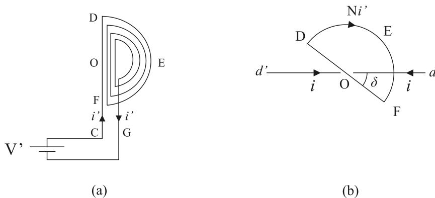
Figure 8.2: (a) Horizontal circuit in semicircle DEF doubled several times over. (b) Angle \delta between the lower horizontal portions of the astatic coil and the straight segment DF of the circuit in semicircle located just below the astatic coil.
