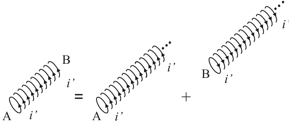
Figure 9.12: A finite current-carrying cylinder AB can be considered as a superposition of two semi-infinite cylinders, one finishing at point A and the other at point B . The current in the cylinder finishing at A flows in the same sense as the current in the finite cylinder AB , while the current in the cylinder finishing at B flows in the opposite sense.
