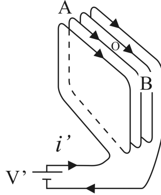
Figure 4.20: A rectangular coil with N turns, with a current intensity i' flowing in each turn. Point O is the midpoint of the upper portion AB .
