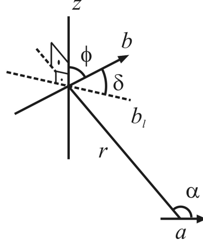
Figure 14.3: The current element a = ids exerts a force on the current element b = i'ds' .
