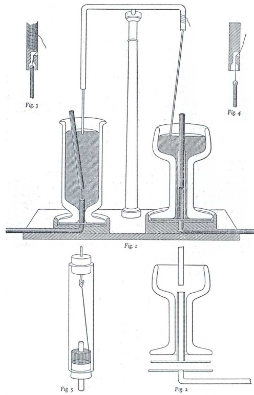
Figure 7.1: Faraday's instruments showing continuous rotation of the extremity of a current-carrying wire around a fixed magnet or the rotation of the extremity of a magnet around a fixed current-carrying wire.
