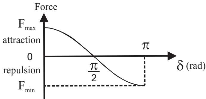
Figure 4.2: Qualitative behavior of the force acting on the mobile conductor BC as a function of the angle \delta in the experiment of figure 3.12.
