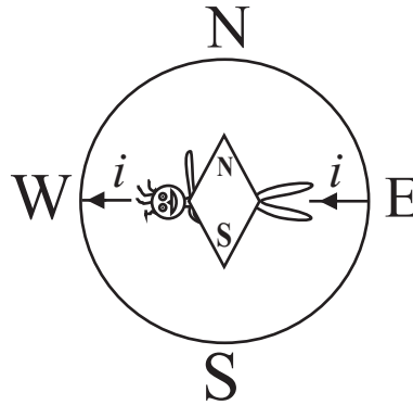
Figure 2.4: In equilibrium, the North pole of a compass will point approximately towards the geographic North pole of the Earth. Ampère’s observer lying on his back and looking at the magnetic needle above it.
