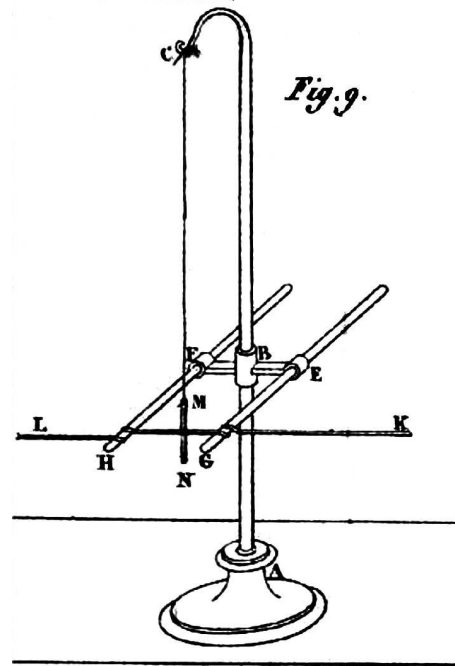
Figure 3.4: A vertical magnetic needle MN can be attracted or repelled by a long horizontal wire KL when there is a constant current in the wire.
