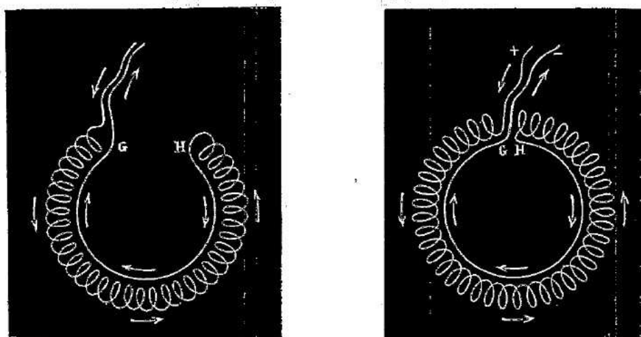
Figure 9.5: (a) When the electrodynamic ring is open, it exerts a net force upon an external current element. (b) When the electrodynamic ring is closed, it exerts no net force upon an external current element.
