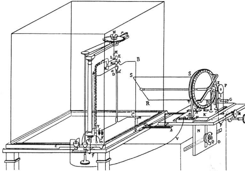
Figure 3.12: Instrument utilized to show the interaction between two conductors having variable orientations. Conductor SR is fixed in the laboratory, having an angular inclination which can be adjusted relative to the vertical direction. Conductor BC is mobile around the vertical axis passing through point D in such a way that it can move towards SR or away from it.
