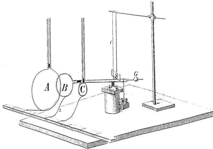
Figure 10.21: Ettingshausen's experiment.
