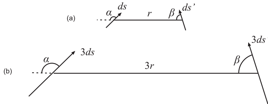
Figure 10.17: (a) Current elements of lengths ds and ds' separated by a distance r . (b) The lengths of both current elements and also the distance between them was multiplied by a single factor (like 3 in this example). When the mutual force between the current elements does not change its intensity, it is said that it follows the law of similarity. In this situation it can be concluded that n = 2 .
