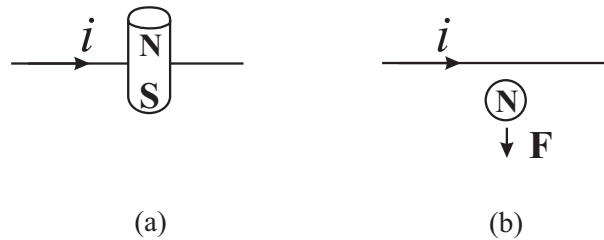
Figure 3.5: (a) Simplified representation of figure 3.4, seen sideways. (b) The experiment seen from above. The letter F represents the force exerted by the horizontal wire on the vertical needle.
