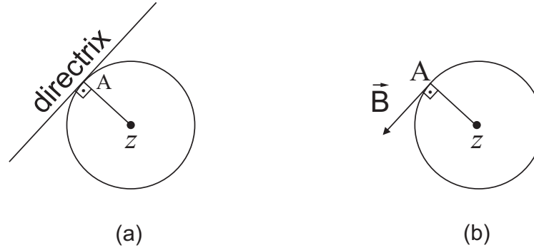
Figure 10.4: (a) Directrix due to an infinite straight wire carrying a current i along the positive z direction, orthogonal to the plane of the paper. (b) Magnetic field \vec{B} due to this current-carrying wire.
