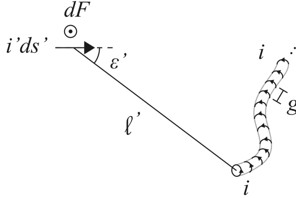
Figure 10.7: Force dF acting on a current element i'ds' and being due to an indefinite solenoid.
