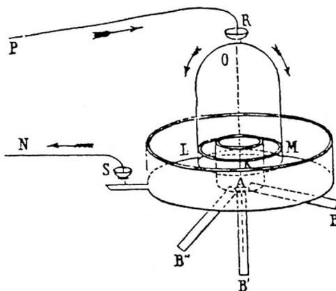
Figure 7.3: The horseshoe conductor turns around its axis relative to the ground when a constant current flows through it with a magnet placed below the system. The arrows indicate the directions of the current.
