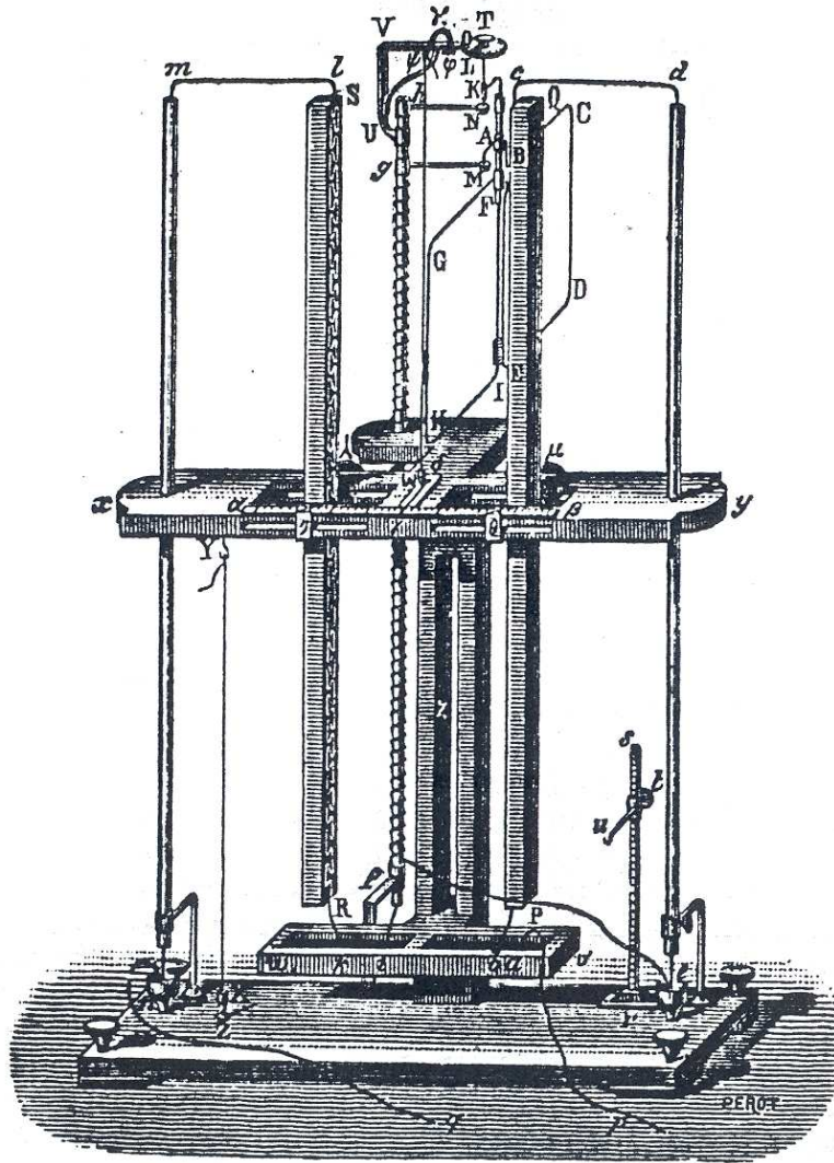
Figure 4.17: Case of equilibrium of the sinuous wire. The fixed sinuous wire is SR , while the fixed vertical wire is QP . The astatic coil ABCDEFGHIM can turn freely around a vertical axis passing through FI , in such a way that the mobile vertical portion GH can move towards SR or away from it.
