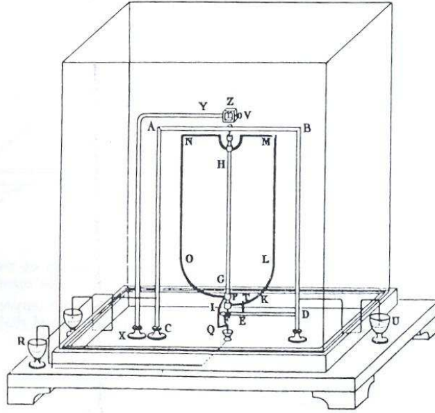
Figure 3.15: Ampère reproduced Ørsted's original experiment utilizing now only current-carrying conductors. In Ampère's original figure 2 of his paper, [Ampère, 1820f], the letters G and H along the central vertical axis do not appear. As these letters were mentioned by Ampère in his paper, they were included here in order to facilitate the comprehension of this experiment. A figure with these letters as they are shown here appeared in [Ampère, 1964, p. 36]. Conductor AB is fixed in the laboratory, while conductor MN is mobile. It can turn freely around the vertical axis ZHGP .
