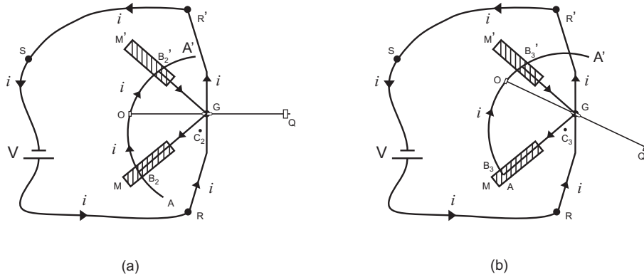
Figure 10.16: (a) Arc B_2B_2' with its center C_2 lying outside the vertical rotation axis GH . After being released from rest it does not remain in equilibrium, rotating around the vertical axis. (b) One of the configurations of the arc during its sliding on the mercury of the troughs. The angle B_2OG is equal the angle B_3OG at the hinge O .
