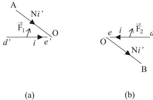
Figure 4.24: (a) \vec{F}_1 represents the attractive force exerted by the half AO of the fixed conductor acting on the lower portion d'e' of the astatic coil which is closer to AO . (b) \vec{F}_2 represents the repulsive force exerted by OB acting on de .
