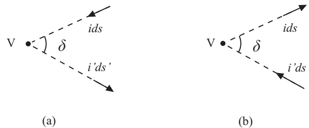
Figure 3.19: Electric currents in the same plane. One of them flows towards a certain point V , while the other flows away from it. According to Ampère, a repulsion should take place between the current elements ids and i'ds' in both situations, (a) and (b).
