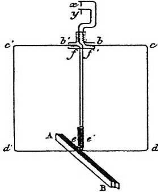
Figure 4.19: Case of equilibrium of anti-parallel currents.
