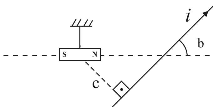
Figure 6.7: A long straight wire located in the vertical plane of the paper, making an angle b with the horizontal. A small horizontal magnetized needle has its center at a distance c to the wire.
