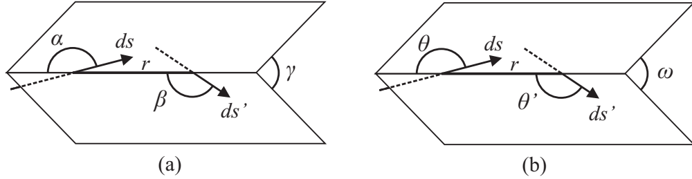
Figure 2.15: Let r be the distance between the midpoints of the current elements of lengths ds and ds' . (a) Representation of the angles \alpha , \beta and \gamma according to Ampère's specifications. Analogous representation of the angles \theta , \theta' and \omega .
