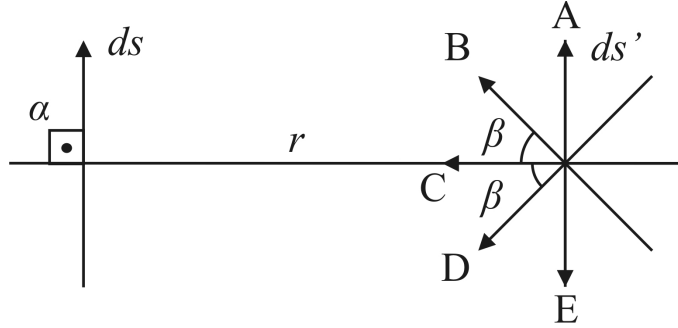
Figure 4.5: Interaction between two current elements located in the same plane. In configurations A and B we have \gamma = 0 rad, in C the angle \gamma is undefined, while in configurations D and E we have \gamma = \pi rad.
