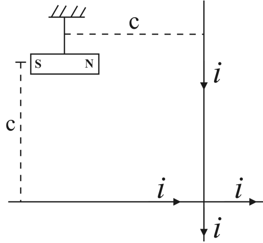
Figure 6.8: A vertical wire and a horizontal wire carry currents of the same intensity, being at equal distance c from the center of a small cylindrical magnet which has its center in the same vertical plane formed by these wires. The magnet can turn in the horizontal plane around the vertical thread holding it.
