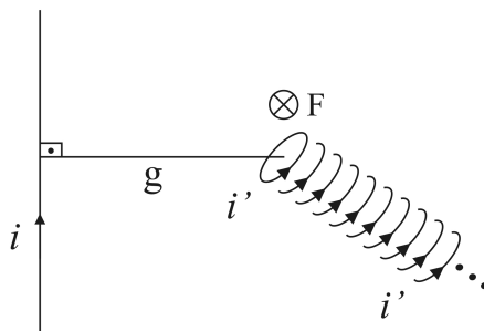
Figure 9.10: Force F exerted by a straight wire on a semi-infinite cylinder.
