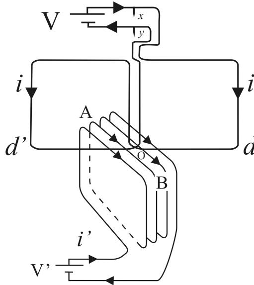
Figure 4.21: Rectangular coil below an astatic coil. The rectangular coil is fixed in the laboratory, while the mobile astatic coil can turn freely around its vertical axis of symmetry.
