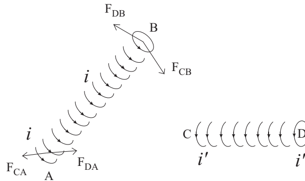
Figure 9.13: Electrodynamic cylinders AB and CD .
