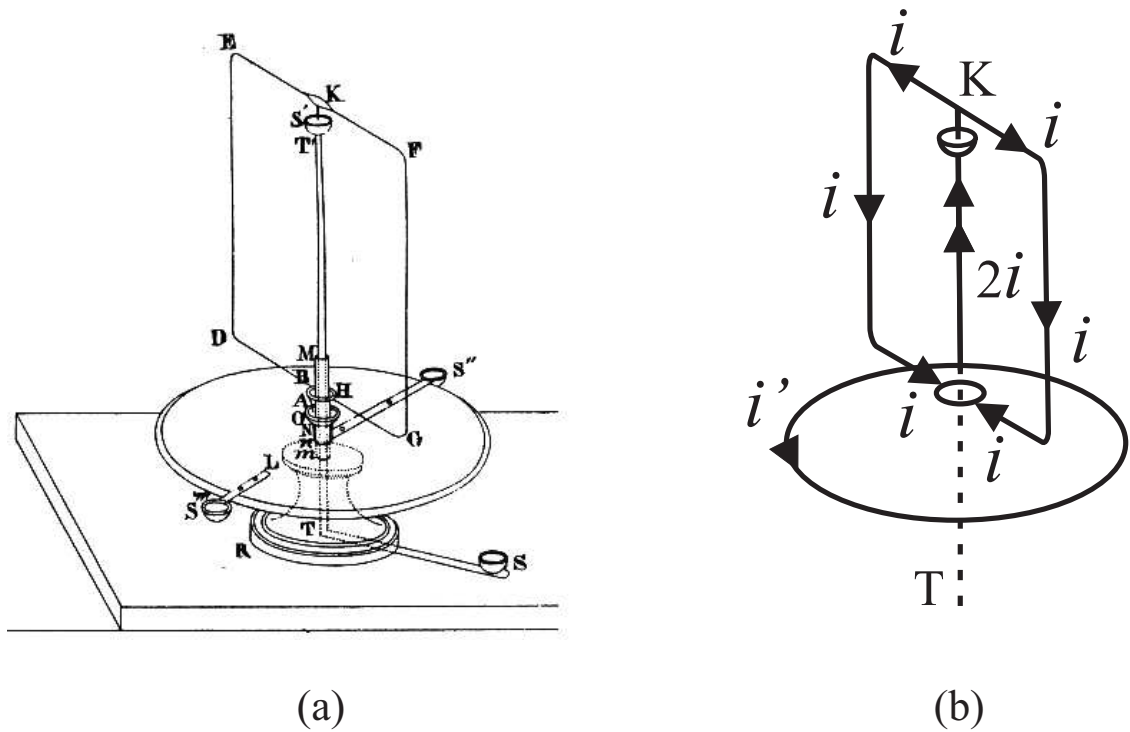
Figure 7.16: (a) Case of equilibrium of the nonexistence of continuous rotation. (b) Directions of the currents in Ampère's crucial experiment.
