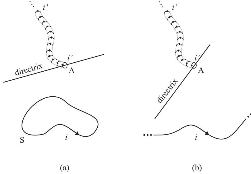
Figure 10.8: (a) Directrix due to a closed circuit of arbitrary shape acting passing through the extremity of an indefinite solenoid located at an arbitrary point in space. (b) Directrix due to a circuit of arbitrary shape extending indefinitely in both directions passing through the extremity of an indefinite solenoid.
