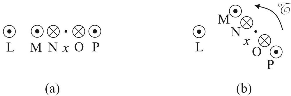
Figure 8.5: Illustration of figure 8.4 as seen from above. (a) Astatic coil in equilibrium, aligned with the rectilinear vertical conductor AB . (b) Astatic coil removed from the equilibrium configuration and torque \tau acting on it, forcing the astatic coil to return to the equilibrium configuration.
