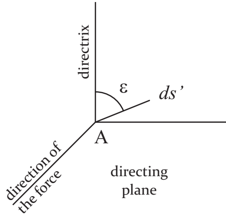
Figure 10.2: The directing plane and the directrix orthogonal to this plane, with the angle \varepsilon between the directrix and the direction of the current element i'ds' .
