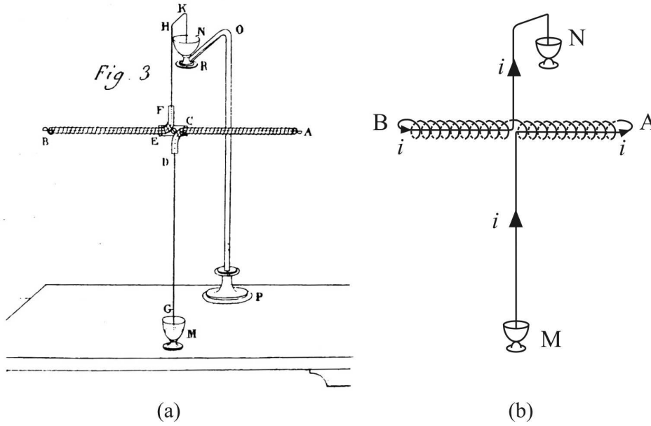
Figure 3.11: (a) Ampère's helix. (b) Our reproduction of this figure indicating the current sense in this experiment.
