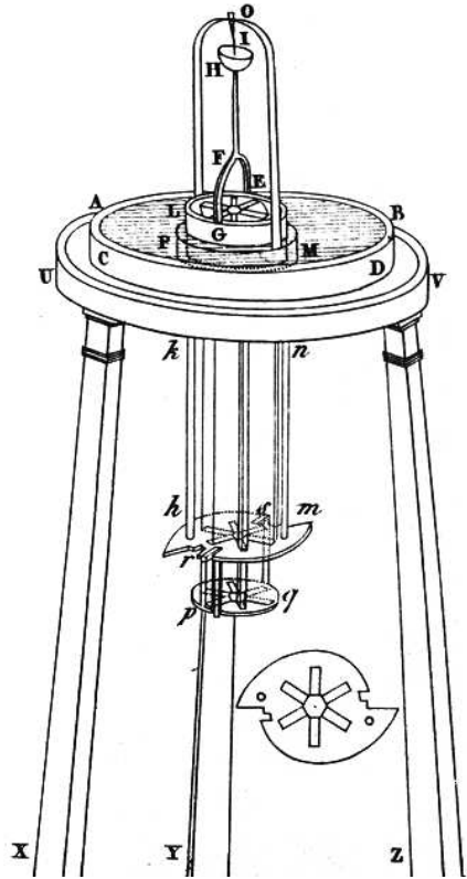
Figure 7.4: Another instrument with which Ampère obtained continuous rotation.
