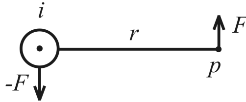
Figure 13.1: A long straight wire normal to the plane of the paper, with a current i coming out of the paper. The arrows indicate the forces exerted between a North pole p of the magnetized needle and the current-carrying wire, according to Faraday's conceptions.
