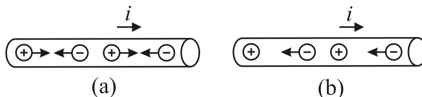
Figure 2.1: (a) According to Ampère, in a current-carrying wire there should be positive and negative charges moving in opposite directions relative to the wire. (b) Modern conception of current in a metal wire with the positive ions at rest relative to the wire, while only the negative electrons move relative to the wire.
