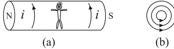
Figure 5.2: Electric currents flowing on the surface and inside a cylindrical magnet, according to Ampère's initial conception of magnetism.
