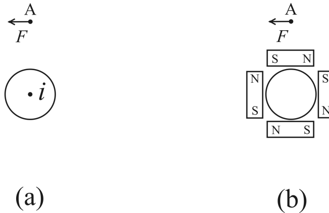
Figure 18.2: Biot and Savart's explanation of Ørsted's experiment.
