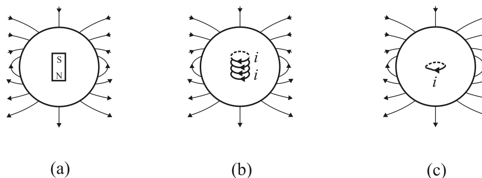
Figure 10.24: (a) In the model of Humboldt and Biot a small magnetic dipole located at the center of the Earth inclines the dip needles located at the surface of the Earth. (b) Savary obtained the same effect replacing the magnetic dipole by an electrodynamic cylinder. (c) Ampère obtained the same effect replacing the magnetic dipole by a small planar loop of arbitrary shape.
