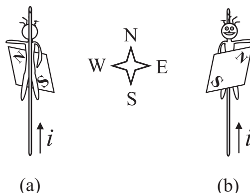
Figure 2.2: Representation of Ampère's observer in Ørsted's experiment. In both cases the observer is located between the current-carrying wire and the magnetic needle. In case (a) the needle is located below the wire, analogous to figure 1.3, while in case (b) the needle is above the wire, as in figure 1.4. When there is no current in the wire, the needle points in the North-South direction along the magnetic meridian. When the current flows in the wire from the South towards the North, then the North pole of the needle moves towards the left side of the observer in both cases.
