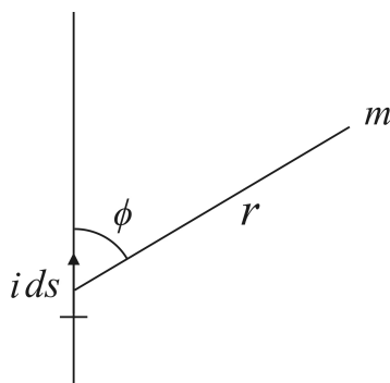
Figure 6.3: A particle of austral or boreal magnetism is represented by the letter m .
