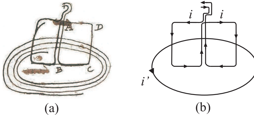
Figure 7.15: Directions of the currents in Ampère's crucial experiment.
