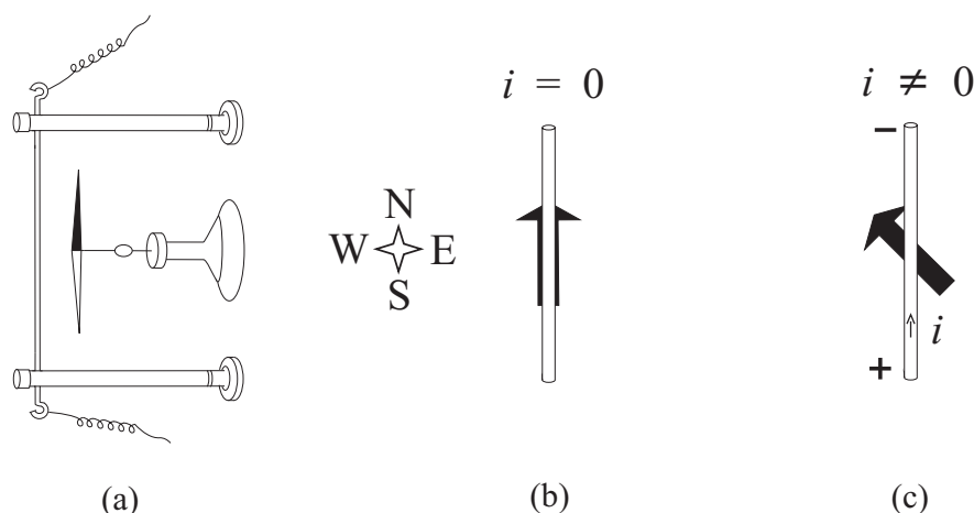
Figure 11.1: Representation of Ørsted's experiment with the horizontal wire above the magnetic needle. In (a) and (b) the needle points along the magnetic meridian while there is no electric current in the wire. In (c) there is a constant current flowing from the South towards the North. The needle is deviated from the magnetic meridian, with its North pole going westward.
