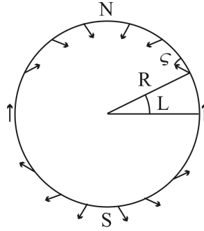
Figure 10.23: Dip angle \zeta as a function of the latitude angle L . The letter R indicates the Earth's radius.
