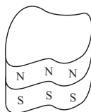
Figure 10.13: A magnetic dipole layer.
