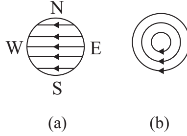
Figure 5.1: Possible representation of the supposed terrestrial electric currents according to Ampère. (a) Currents over the surface of the Earth. (b) Concentric currents inside the Earth along its magnetic equatorial plane, with the North pole above the paper and the South pole below the paper.
