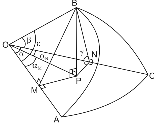
Figure 7.18: Spherical triangle.
