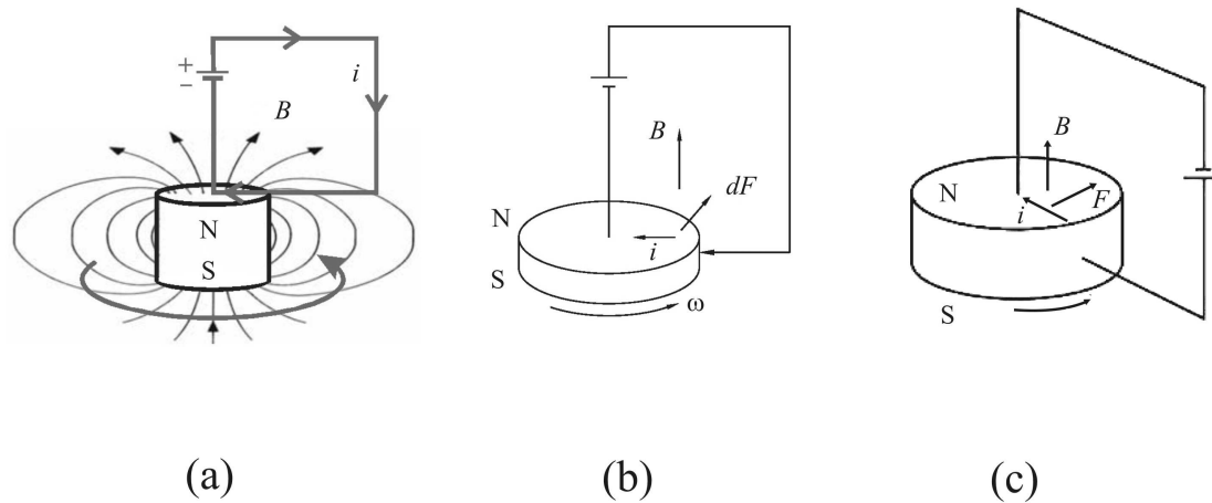
Figure 21.11: Modern explanations for the rotation of a magnet around its axis utilizing his own magnetic field B and the force exerted by this magnetic field acting on a current flowing inside the magnet.
