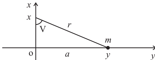
Figure 6.5: A current-carrying wire along the x axis with a magnetic particle m at a distance a to the wire.
