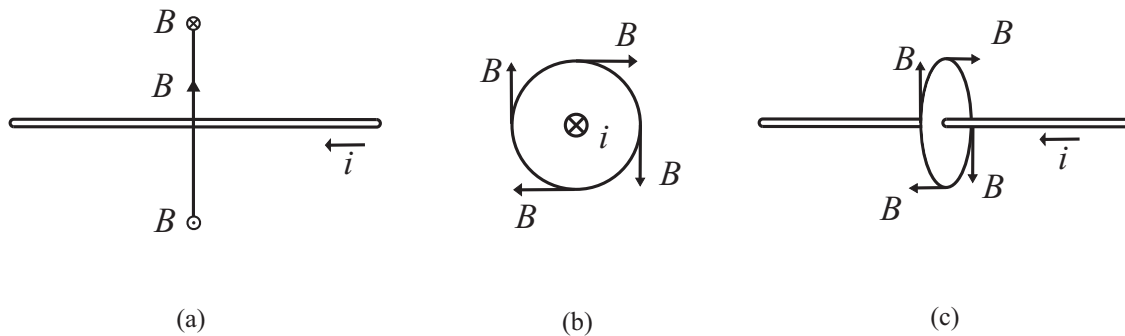
Figure 20.1: Magnetic field around a long current-carrying wire. (a) Lateral view. (b) View orthogonal to the wire. (c) View in perspective.
