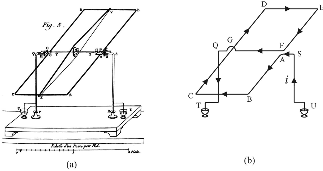
Figure 3.14: (a) Rectangular current-carrying loop which is oriented by terrestrial magnetism, in analogy with a dip needle. (b) Our figure indicating the sense of the electric current in this experiment.
