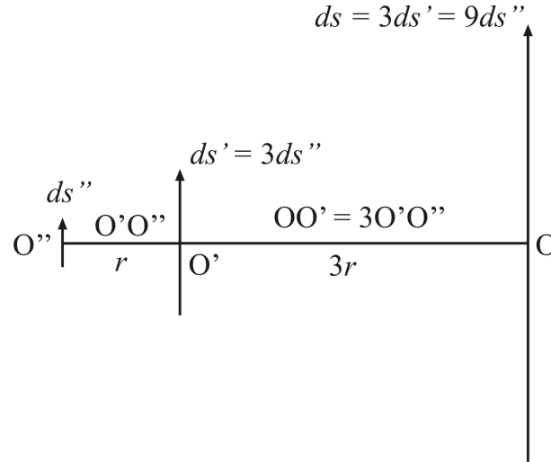
Figure 10.18: Three parallel current elements with their dimensions and distances satisfying the relation ds/ds' = ds'/ds'' = OO'/O'O'' = 3 .
