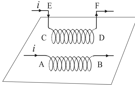
Figure 4.7: Interaction between two helices.
