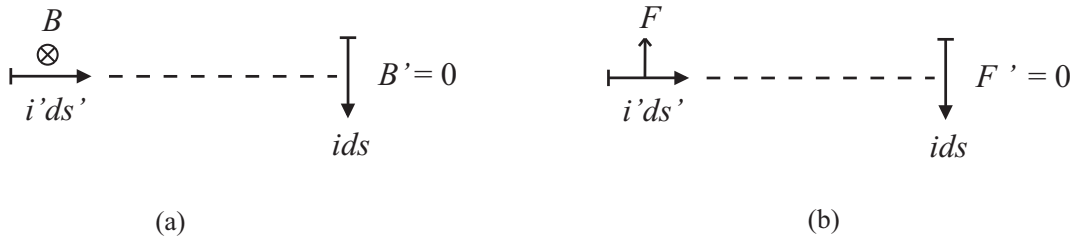
Figure 20.9: (a) Magnetic fields generated by the current elements. (b) Forces acting on the current elements.
