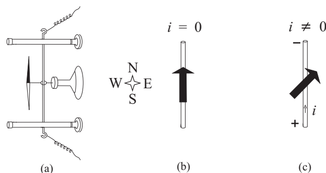
Figure 1.4: Representation of Ørsted's experiment with the horizontal wire below the magnetic needle. In (a) and (b) the needle points along the magnetic meridian while there is no electric current in the wire. In (c) there is a constant current flowing from the South towards the North. The needle is deviated from the magnetic meridian, with its North pole going eastward.
