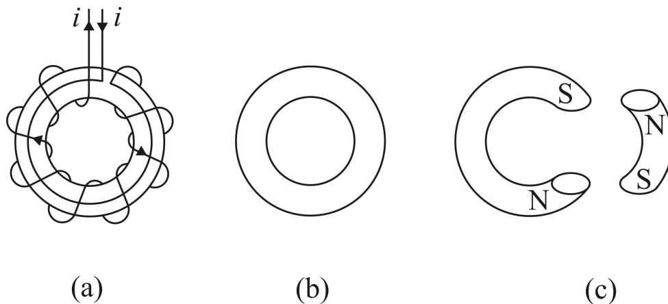
Figure 9.1: (a) A constant current flows through a toroidal wire coiled around an unmagnetized steel ring. (b) The wire is removed and the ring does not interact with a compass needle. (c) The ring is broken into pieces and each piece behaves like a small magnet, interacting with a compass needle.
