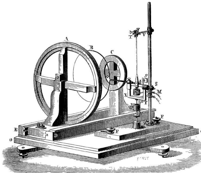
Figure 10.22: Felici's experiment.
