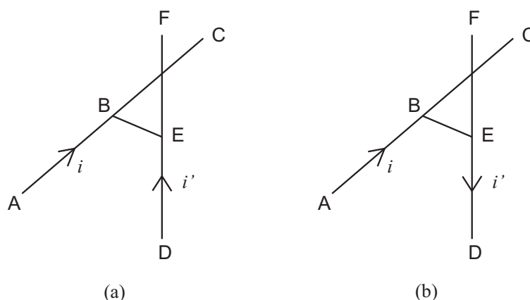
Figure 7.11: (a) Attraction between current-carrying conductors AB and DE . (b) Repulsion between current-carrying conductors AB and DE .
