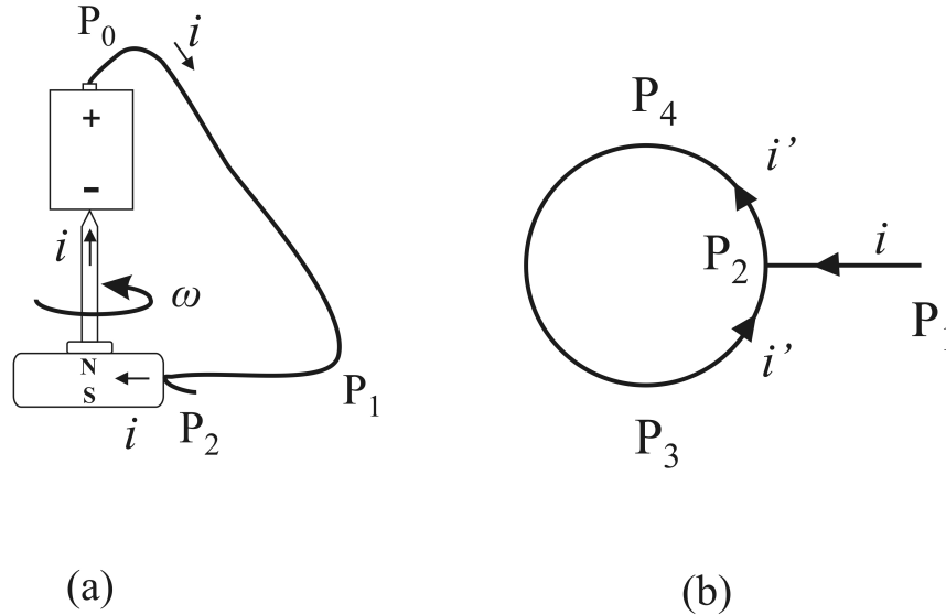
Figure 21.12: (a) Magnet and screw rotate around the common axis. (b) Configuration as seen from above indicating the current i generated by the battery and flowing in the sense P_1P_2 , together with the net effect i' of all molecular currents due to the magnet itself flowing in the sense P_3P_2P_4 .
