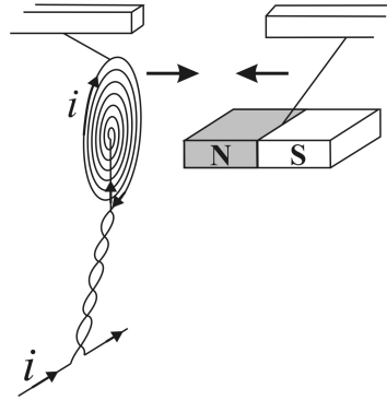
Figure 3.7: Attraction between a current-carrying wire bent in a spiral and a magnetized bar. The remainder of the closed circuit connecting the extremities of the wire to the battery is not shown. The wire connecting the spiral to the upper support is an insulator.
