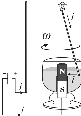
Figure 7.2: Illustration of the main elements of Faraday's instrument in which the extremity of a wire carrying a current i rotates with angular velocity \omega around a magnet NS .
