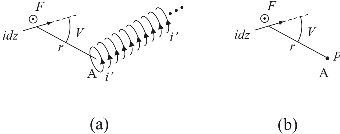
Figure 9.6: (a) Force F exerted on a current element by a semi-infinite cylinder. By action and reaction, the current element exerts an equal and opposite force on the cylinder. (b) This electrodynamic cylinder behaves like the supposed magnetic pole of Biot and Savart located at the extremity A of the cylinder, as the current element idz exerts the same force on the electrodynamic cylinder and on the magnetic pole.
