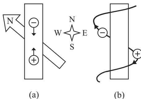
Figure 11.2: (a) Ørsted's experiment. (b) His interpretation of this observation in which he supposed positive and negative electricities describing helical paths around the wire and propelling the magnetic poles of the magnet. The arrows indicate the directions of motion of the supposed positive and negative charges moving (a) inside and (b) outside the wire.
