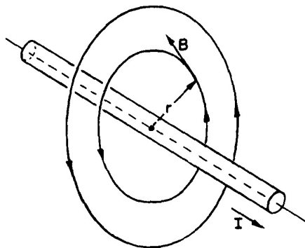
Figure 20.2: Magnetic field around a current-carrying wire, according to Feynman.
