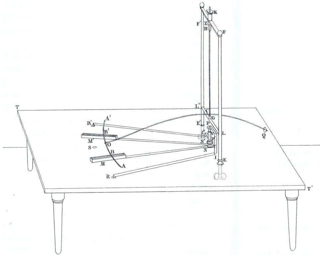
Figure 10.14: Case of equilibrium of the nonexistence of tangential force.
