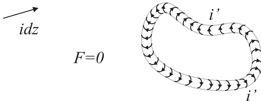
Figure 9.9: There is no interaction between a closed solenoid and an external current element.
