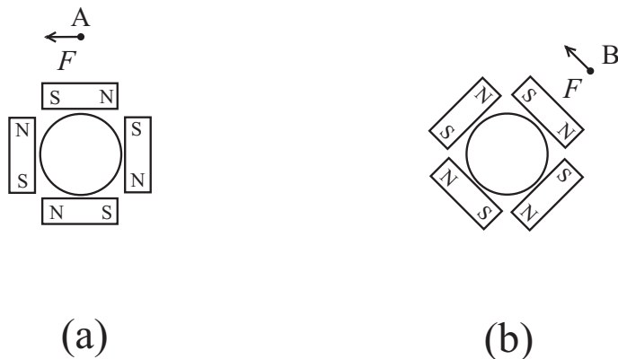
Figure 18.4: (a) Magnetization of the wire when the magnetic pole is located at point A. (b) Magnetization of the wire when the magnetic pole is located at point B.
