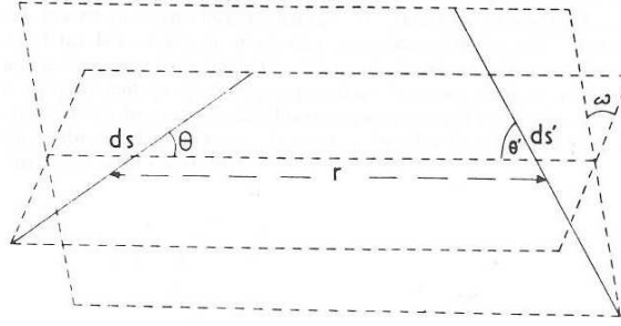
Figure 2.16: Representation of the angles \theta , \theta' and \omega according to Tricker.
