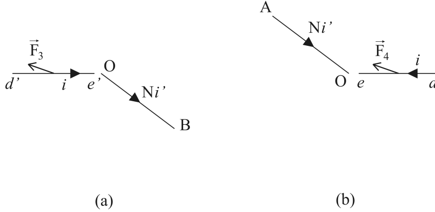
Figure 4.25: (a) \vec{F}_3 represents the repulsive force exerted by the half OB of the fixed conductor acting on the farthest lower portion d'e' of the astatic coil. (b) \vec{F}_4 represents the attractive force exerted by AO acting on de .
