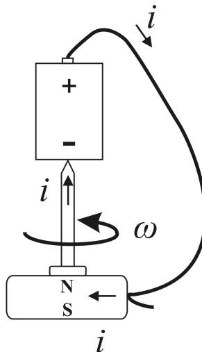
Figure 7.9: A magnetized screw rotates with angular velocity \omega , together with the magnet NS attached to it, around the axis of the battery, when there is a constant current i flowing in the circuit. There is a sliding contact between the wire and the magnet.
