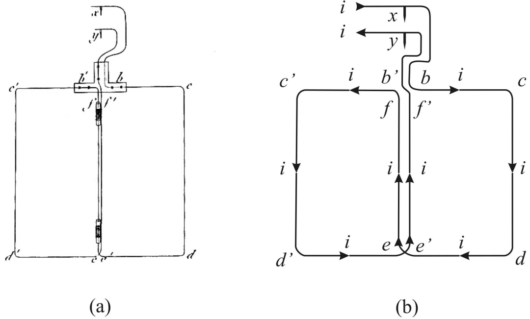
Figure 4.16: (a) Astatic coil indifferent for terrestrial magnetism. This vertical coil can rotate around the vertical symmetry axis passing through x and y . (b) Our representation of the sense of the current along this astatic coil. It flows clockwise in bcdef and anti-clockwise in b'c'd'e'f' .
