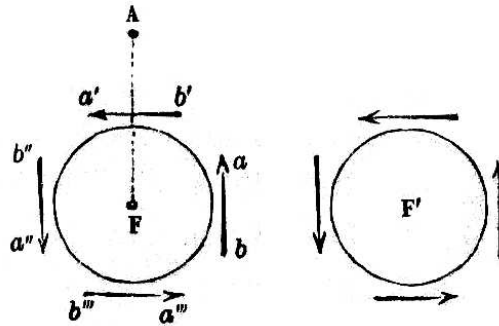
Figure 21.1: Biot and Savart's explanation of Ampère's experiment.
