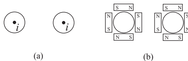
Figure 21.2: (a) Two straight wires carrying currents in the same direction and attracting one another. (b) Biot and Savart's explanation of this effect supposing the magnetization of both wires and the interaction of the supposed magnets distributed around the cross sections of both wires.
