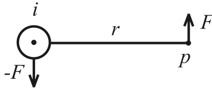
Figure 20.5: Primitive couple according to Faraday's conceptions.
