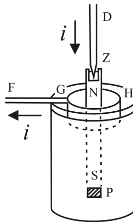
Figure 7.7: The magnet NS floats in mercury with the help of the counterweight P in its lower extremity. At the upper extremity of the magnet there is a cavity Z filled with mercury. The electric current i flows down along DZ , leaving laterally along GF . There is a metal ring GH connected to the mercury. In this configuration the magnet turns around its axis relative to the ground.
