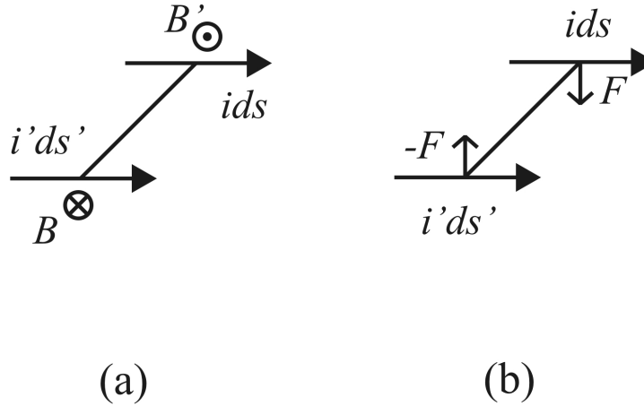
Figure 20.7: (a) Magnetic field B' generated by the current element i'ds' and acting on the current element ids . There is a component of this magnetic field orthogonal to the paper, leaving it. Also shown is the magnetic field B generated by ids and acting on i'ds' , with a component orthogonal to the paper, penetrating it. (b) forces generated by these magnetic fields.
