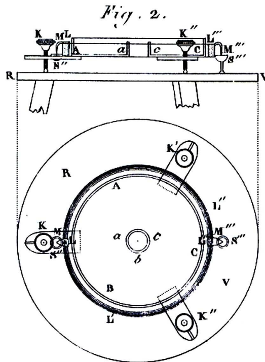
Figure 7.17: Circular current-carrying coil located at the base of the astatic coil of figure 7.16.
