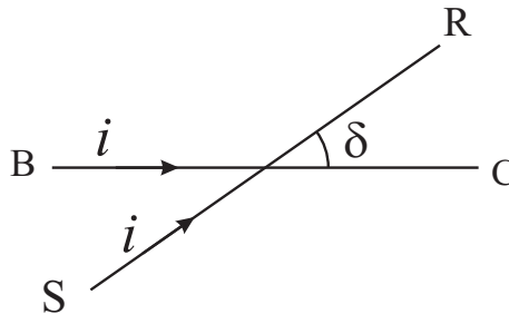
Figure 4.1: This illustration presents the experiment of figure 3.12 as seen along the straight line connecting the centers of conductors SR and BC . Conductor SR is fixed in the laboratory, while conductor BC is mobile, so that it can move towards SR or away from it.
