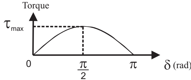
Figure 3.17: Qualitative behavior of the torque acting on the mobile circuit MN as a function of the angle \delta in the experiment of figure 3.15.
