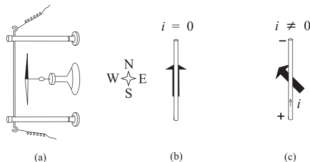
Figure 1.3: Representation of Ørsted's experiment with the horizontal wire above the magnetic needle. In (a) and (b) the needle points along the magnetic meridian while there is no electric current in the wire. In (c) there is a constant current flowing from the South towards the North. The needle is deviated from the magnetic meridian, with its North pole going westward.
