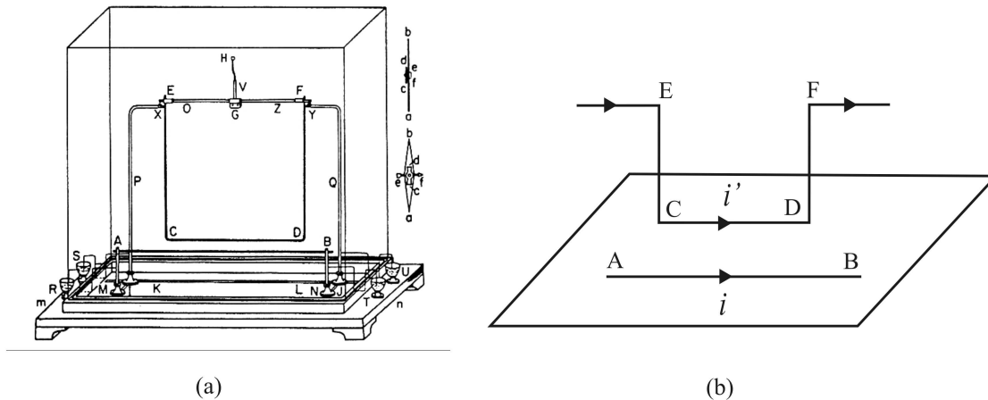
Figure 3.10: (a) Ampère’s demonstration that parallel straight wires carrying currents in the same sense attract one another, repelling when the currents flowed in opposite senses. Conductor AB is fixed in the laboratory, while the mobile conductor CD can turn around the horizontal axis EF , moving towards AB or away from it. The straight segments AB and CD are initially in the same horizontal plane, with the axis EF vertically above CD . (b) Our representation of this experiment, indicating the current senses.
