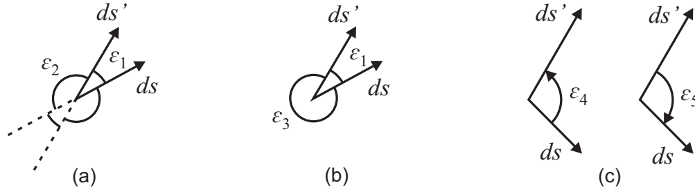
Figure 2.11: There are several ways of defining the angle between two current elements of directed lengths ds and ds' .
