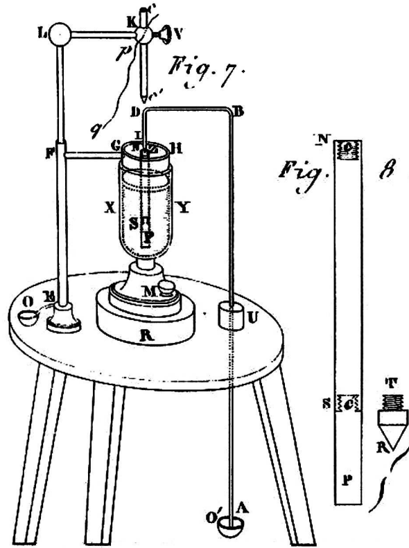
Figure 7.8: With this instrument Ampère was the first scientist to obtain a continuous rotation of a magnet around its axis, a phenomenon Faraday considered improbable to take place.
