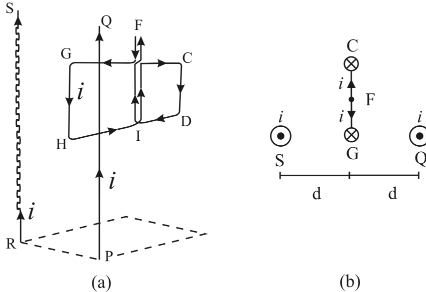
Figure 4.18: (a) Schematic representation of the direction of the current in the experiment of figure 4.17. (b) Case of equilibrium of the sinuous wire seen from above.
