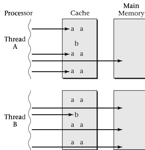
Figure 3.4 When a processor has been executing thread A for a while, the cache will mostly hold thread A's values, and the cache hit rate may be high. If the processor then switches to thread B, most memory accesses will miss in the cache and go to the slower main memory.
