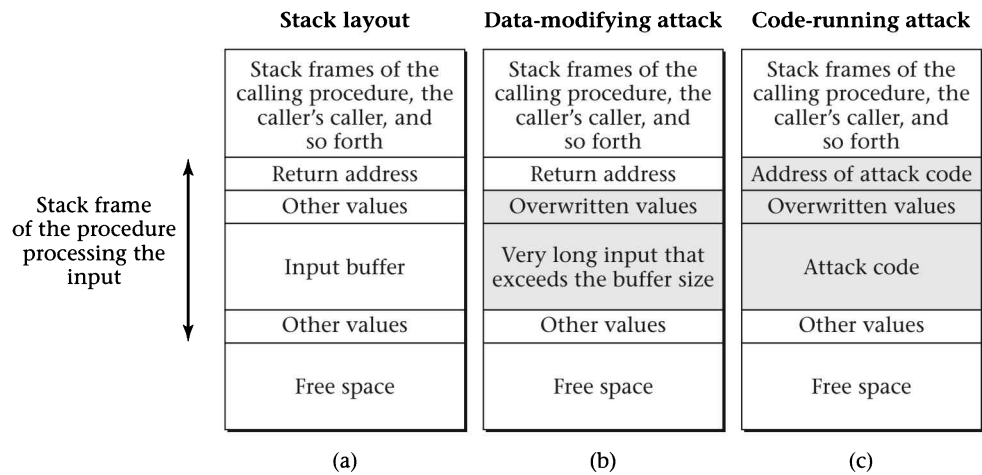
Figure 11.4 If input is allowed to overflow the amount of memory allocated on the stack for an input buffer, it can overwrite other data values, as shown in part (b), or the return address, as shown in part (c). In the latter case, the modified return address can point to attack code included in the oversized input.
