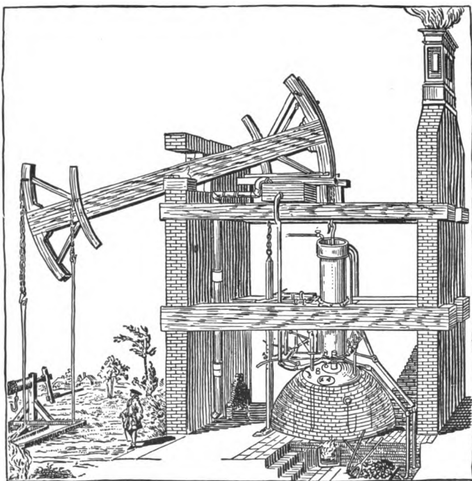
NEWCOMEN'S ENGINE
